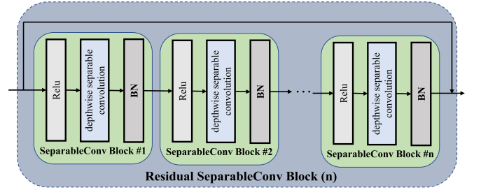
Fig. 4. The network architecture of “Residual SeparableConv block (n)” used in the multi-scale module, where n denotes the number of the separableConv block used in this architecture.
