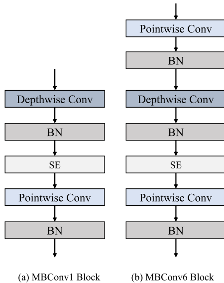
Fig. 3. The network architecture of the MBConv1 Block and MBConv6 Block used in the pre-processing module and MBConv block module.
