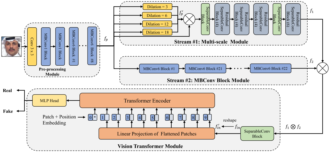
Fig. 2. The network architecture of the proposed method. It includes four modules: pre-processing module, multi-scale module, MBConv block module and vision transformer module. The symbol Dilation = N denotes the dilation rate is N . The symbol \otimes denotes the operation of concatenation.
